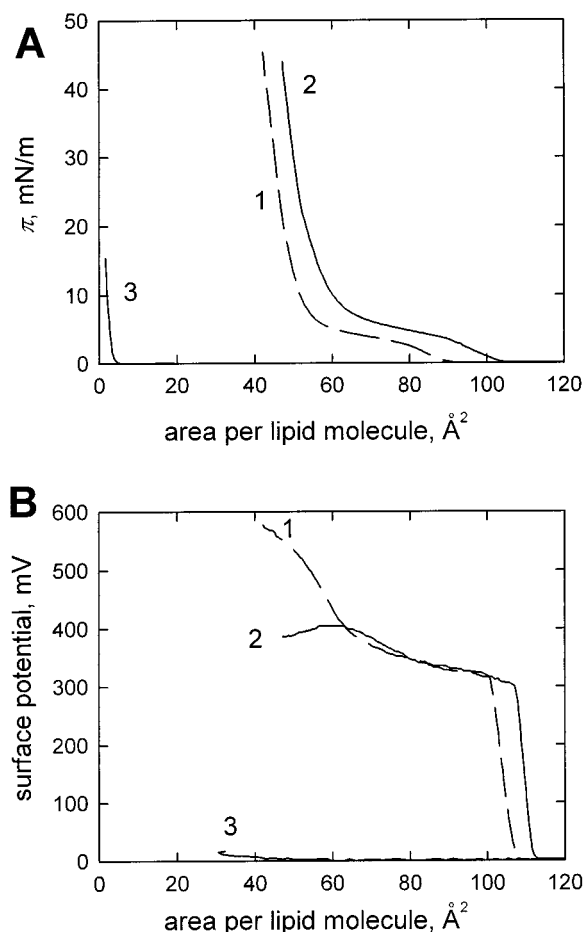
FIGURE 1 Surface pressure ( A ) and surface potential ( B ) versus area per lipid molecule for DPPC monolayer spread on the subphase without gramicidin (curve 1) and in the presence of 10^{-7} M gramicidin (curve 2). Curve 3 presents the control experiment: 10^{-7} M gramicidin in the subphase without spreading DPPC.
