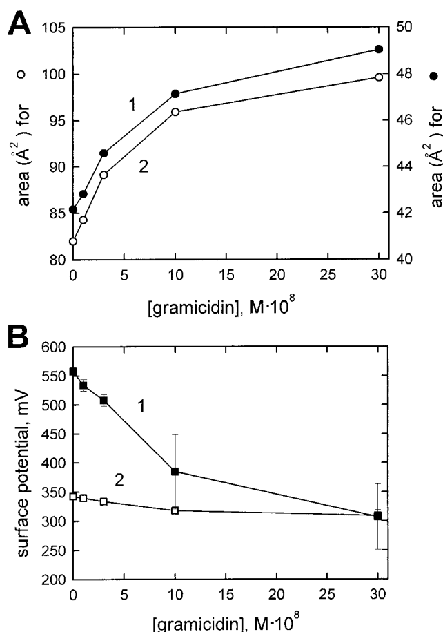
FIGURE 2 Area per DPPC molecule ( A ) and surface potential ( B ) versus gramicidin concentration in the subphase for \pi = 45 mN/m (curve 1) and \pi = 2 mN/m (curve 2).
