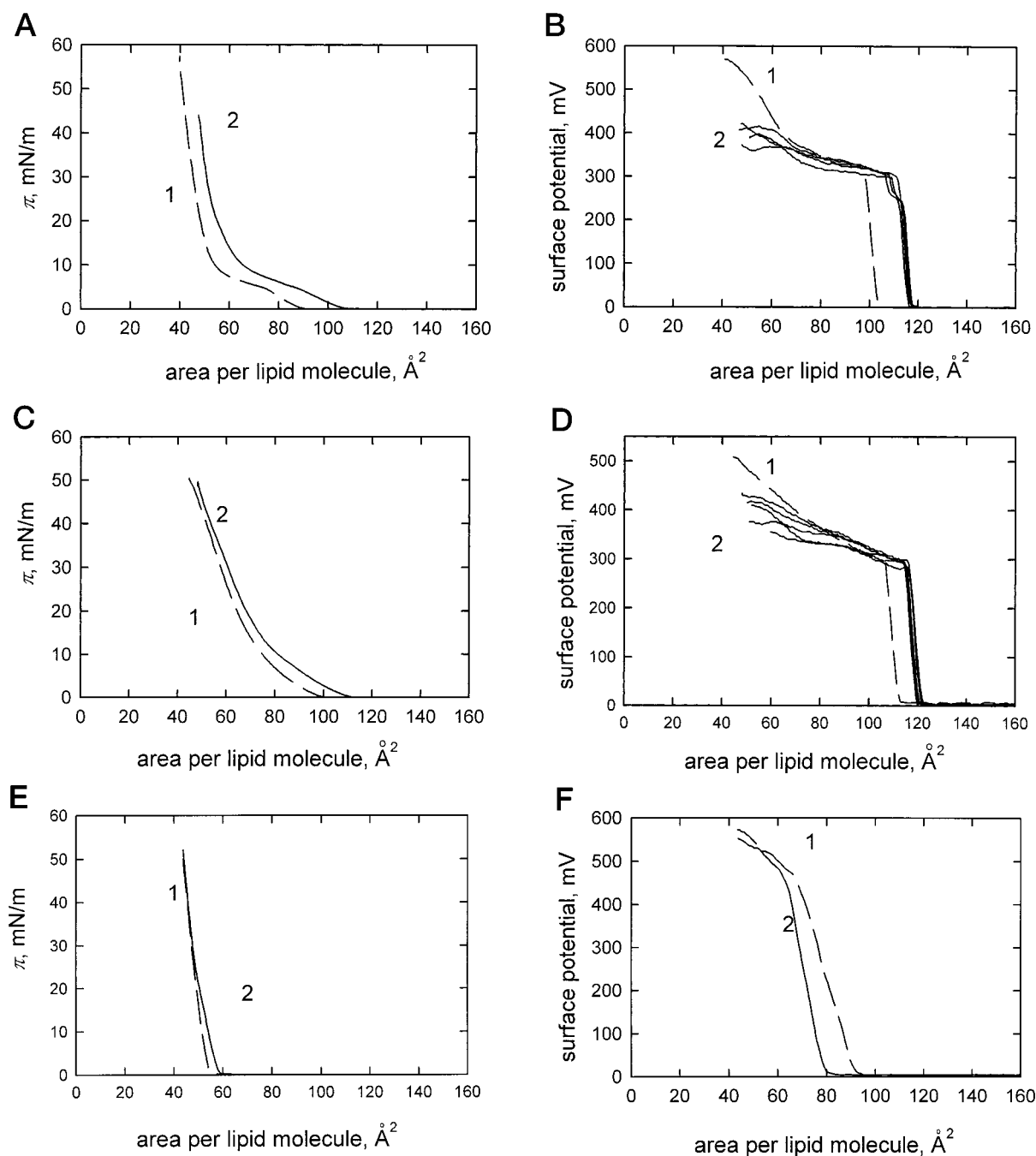
FIGURE 3 Surface pressure (A, C, E) and surface potential (B, D, F) versus area per lipid molecule for DPPC (A, B), DMPC (C, D), and DSPC (E, F) monolayer spread on the subphase without gramicidin (curve 1) and in the presence of 10^{-6} M gramicidin (curve 2). It is seen that in the case of DPPC and DMPC the surface potential-area plots varied significantly from one compression-expansion cycle to another in the presence of gramicidin.
